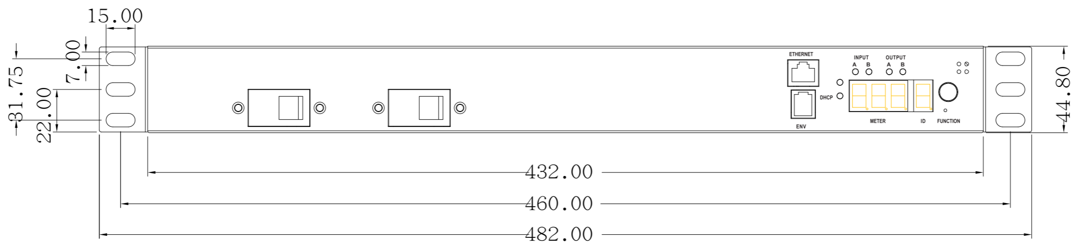
Mounting Bracket
