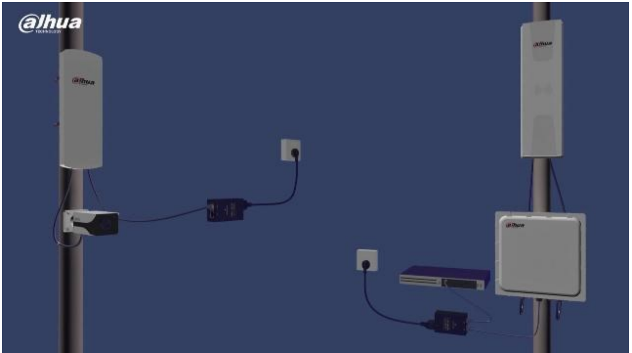
Figure 2-1 DH-PFM88X Overall Installation Diagram
