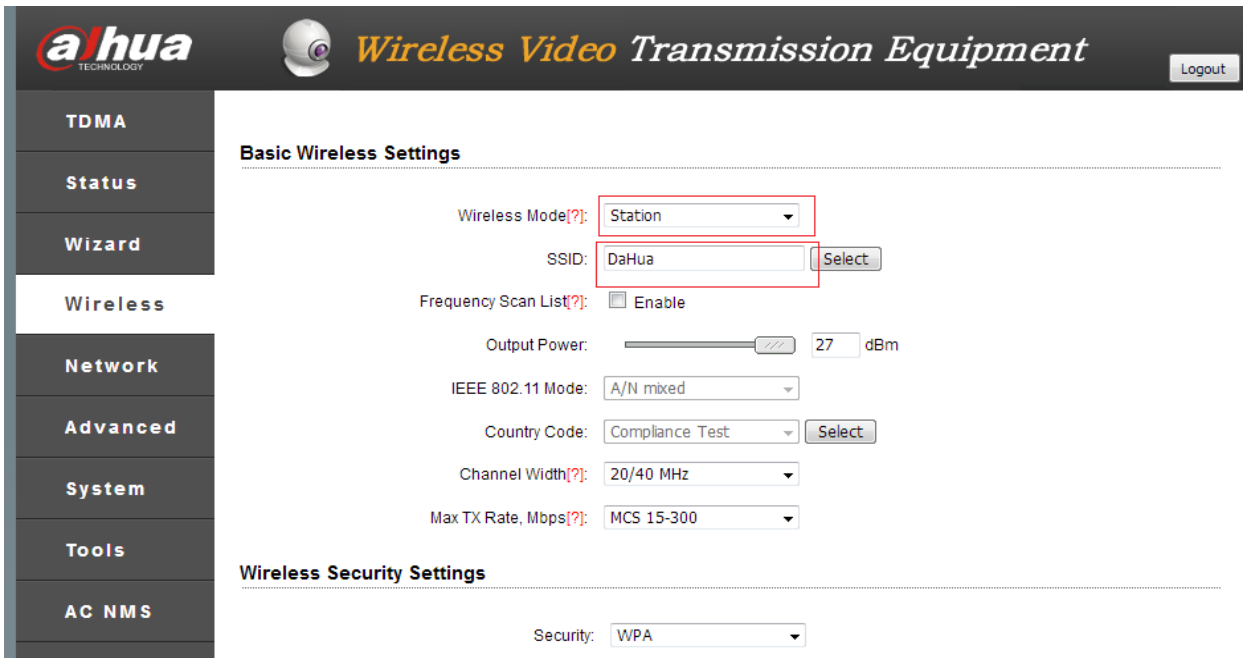
Figure 6-2 Wireless 5.8G Band Searching Page of Client
