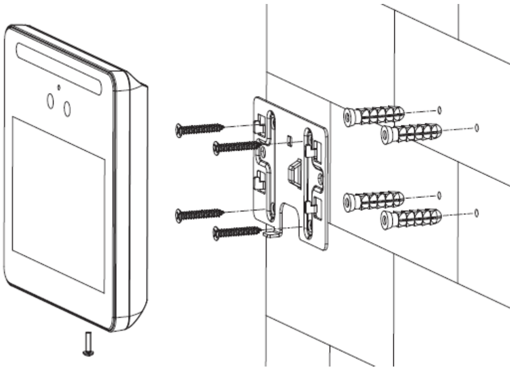
Figure 2-9 Wall installation
