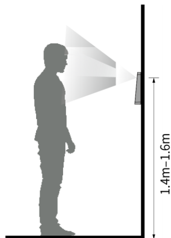
Figure 2-8 Installation height
